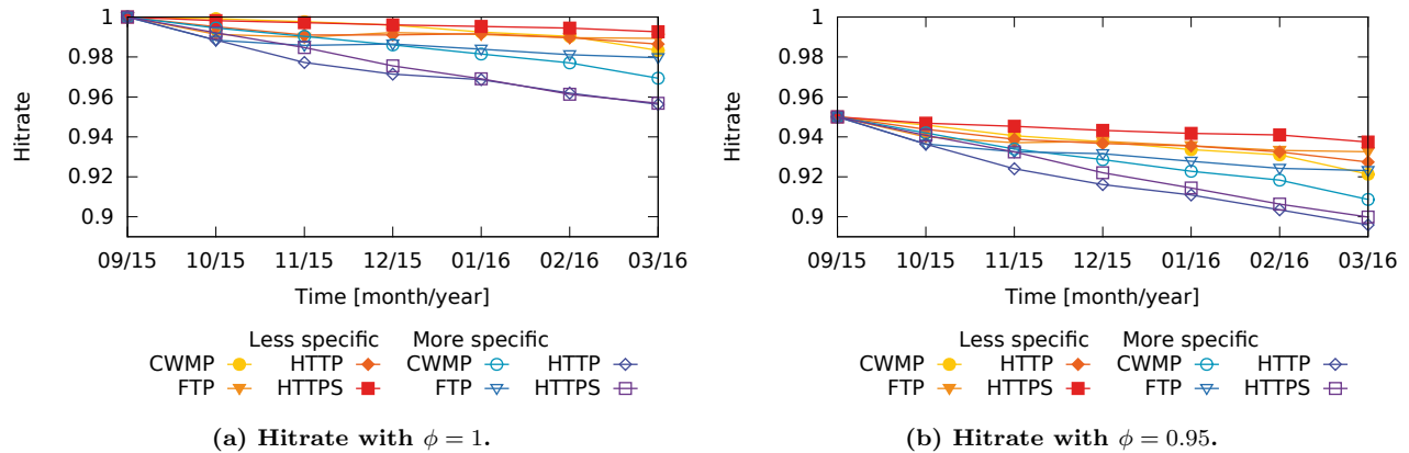
Figure 6: Hitrate of TASS compared to a full scan.
