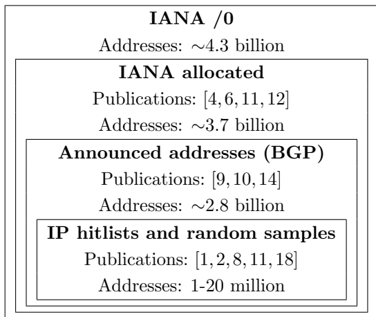
Figure 1: Current scanning strategies and their scoping of the address space.
