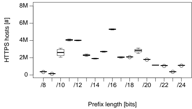
(b) HTTPS for less specific prefixes.
